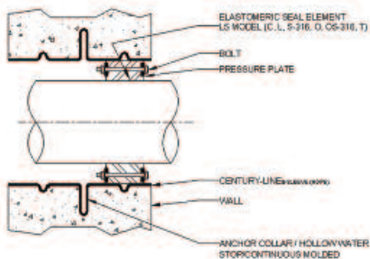
LINK-SEAL® MODULAR SEALS WITH CENTURY-LINE® SLEEVES MANUFACTURED BY PIPELINE SEAL & INSULATOR, INC. HOUSTON, TEXAS, U.S.A. TEL: 800-423-2410 E-MAIL: INFO@PSPI.COM
