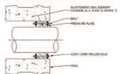
LINK-SEAL® MODULAR SEALS WITH CAST OR CORE DRILLED WALL OPENING MANUFACTURED BY PIPELINE SEAL & INSULATOR, INC. HOUSTON, TEXAS, U.S.A. TEL: 800-423-2410 E-MAIL: INFO@PSPI.COM
