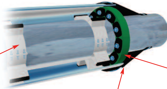
Link-Seal® modular seals with Centering Blocks
