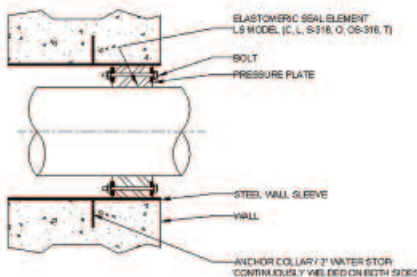
LINK-SEAL® MODULAR SEALS WITH MODEL WS STEEL WALL SLEEVES MANUFACTURED BY PIPELINE SEAL & INSULATOR, INC. HOUSTON, TEXAS, U.S.A. TEL: 800-423-2410 E-MAIL: INFO@PSPI.COM
